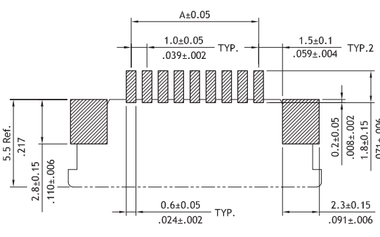
Solder Pad Pattern
