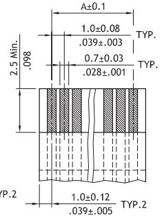
Accommodated FFC
