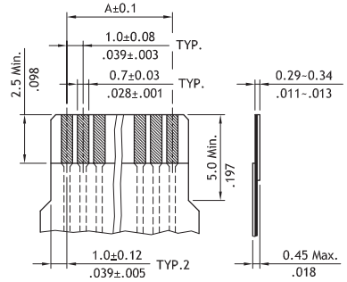
Accommodated FPC
