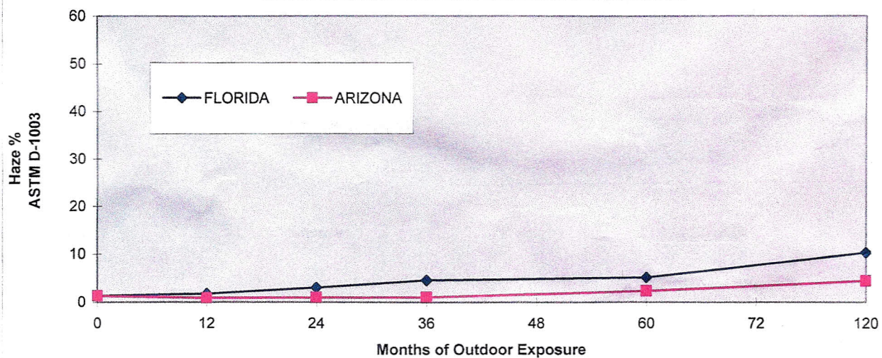
Optical Haze During Outdoor Exposure Testing
