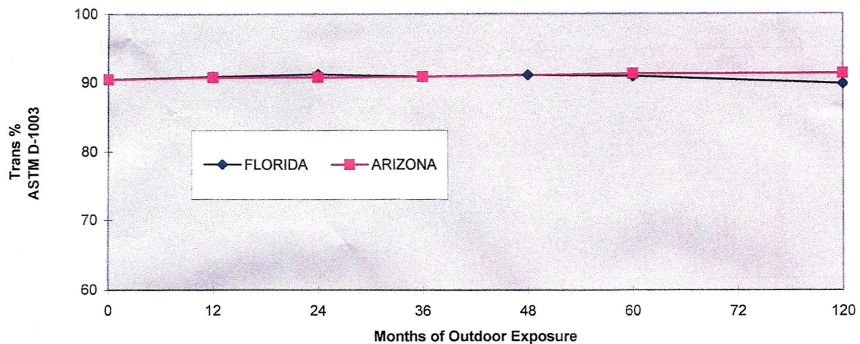
Luminous Transmittance During Outdoor Exposure Testing
